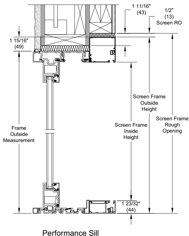
Performance Sill
