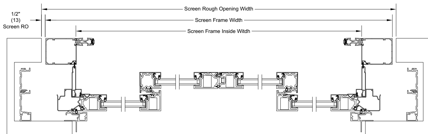
Bi-Parting PXX-XXP
