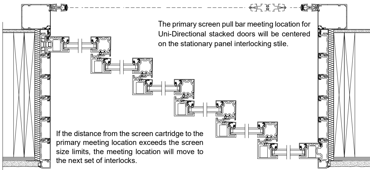
Uni-Directional XXXXXO
