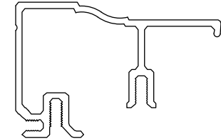
Clad Brick Mould Casing A233 No longer available, replace with A228 or A898
