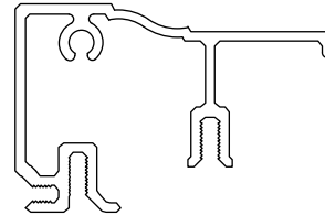
Clad Brick Mould Casing A232 No longer available, replace with A228 or A898
