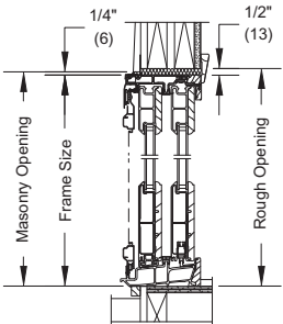
Head Jamb and Sill
