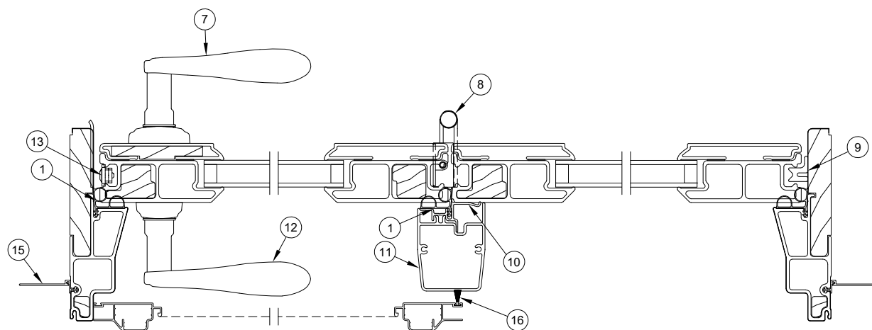
2 Panel Jams - XO - R
