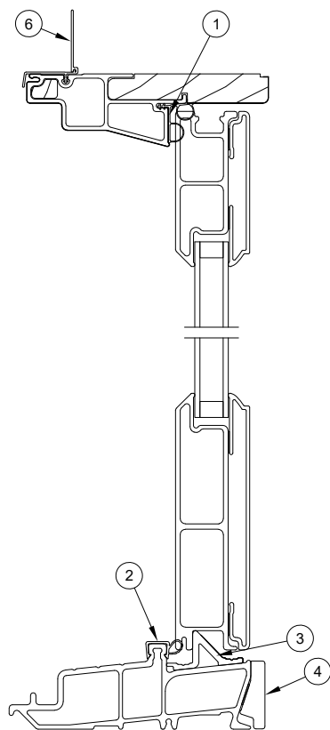
Head Jamb and Sill
