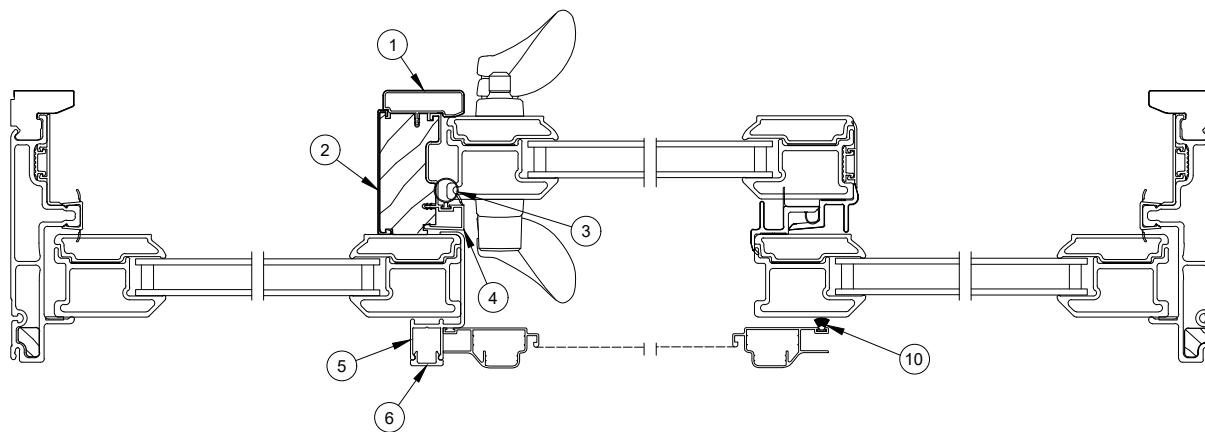
3-Panel Jamb Detail - OXO
