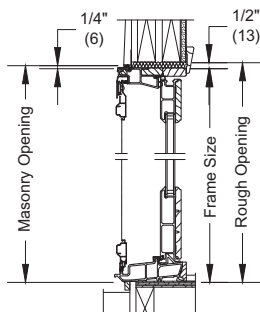
Head Jamb and Sill with Sliding Screen
