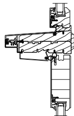
HORIZONTAL MULLION
