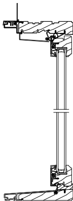
HEAD JAMB AND SILL
