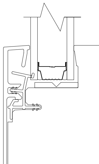
Standard Square Interior Square Exterior
