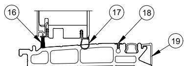
Accessibilty Sill Detail
