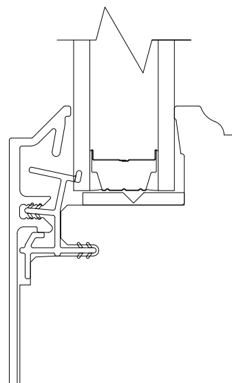
Option Ogee Interior Putty Exterior
