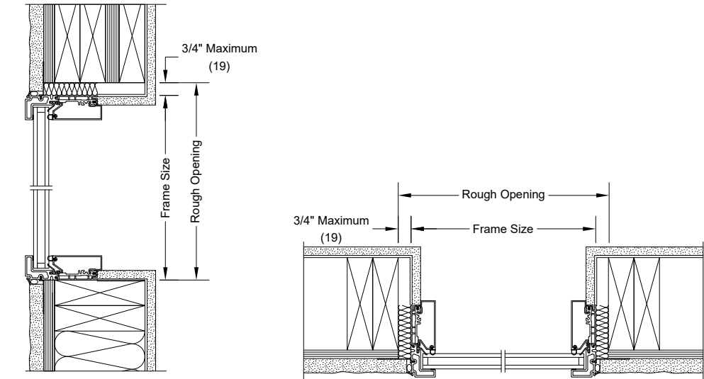
DIRECT GLAZE RECTANGLE HEAD JAMB AND SILL WITH 1 1/4" DUAL PANE
