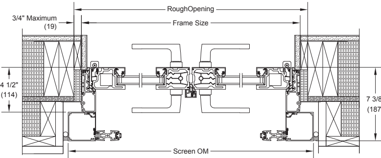
2 PANEL JAMB XX RH WITH SCREEN
