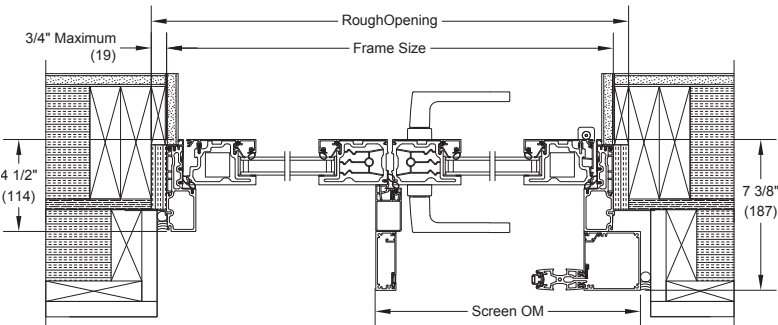
2 PANEL JAMB OX LH WITH RH SCREEN
