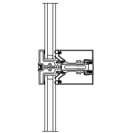
HORIZONTAL MULLION
