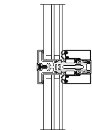
HORIZONTAL MULLION
