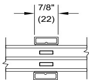
7/8" SDL 1 1/4" Tripane
