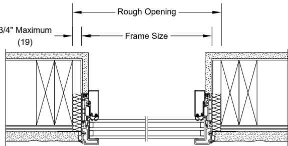
DIRECT GLAZE POLYGON JAMB WITH 1 9/16" TRIPLE PANE
