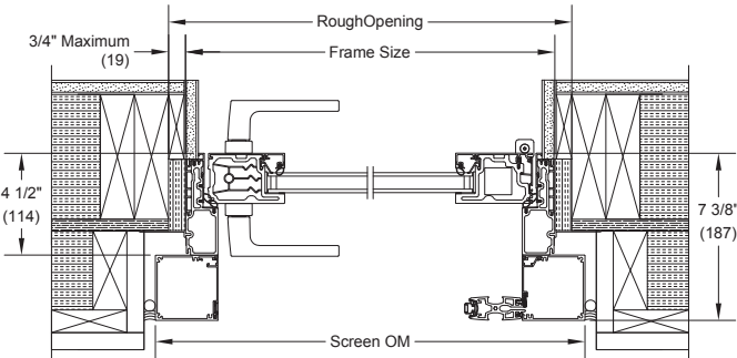
X R JAMB WITH RH SCREEN
