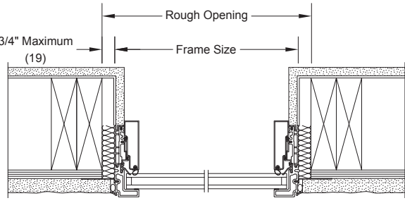
DIRECT GLAZE POLYGON JAMB WITH 1 1/4" DUAL PANE
