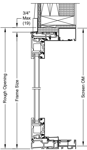
4 9/16" HEAD JAMB AND SILL WITH PERFORMANCE SILL
