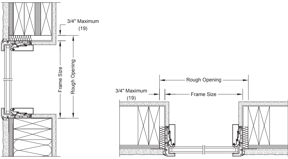
DIRECT GLAZE POLYGON HEAD JAMB AND SILL WITH 1 1/4" DUAL PANE
