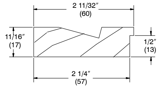
6 13/16" Jamb Extension, W7446
