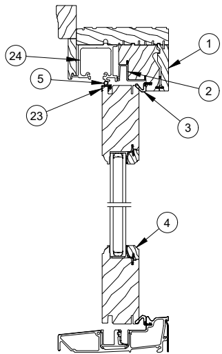
Performance Sill
