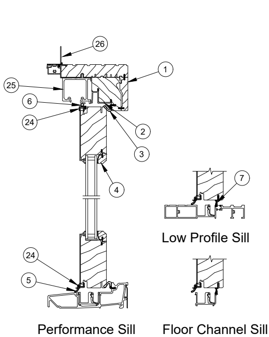
Head Jamb and Sill Details
