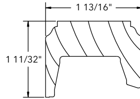
Ogee Astragal Cap, W12708
