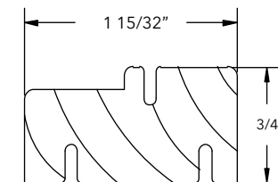
*Tall Frame Cover Support, W12751
