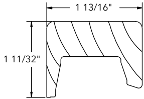
Square Astragal Cap, W12707
