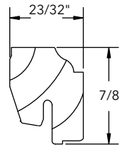
Ogee Glazing Cap, W12367
