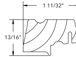
Astragal Base, W12709
