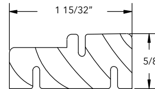
*Mid Frame Cover Support, W12752
