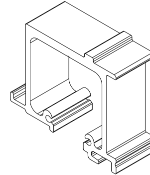
Head Track, A3229
