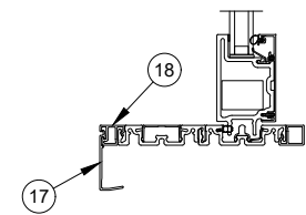
High Performance Sill Option
