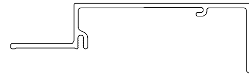
Trim, Pocket, 1 Deep , A3312
