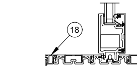
High Performance Sill Option
