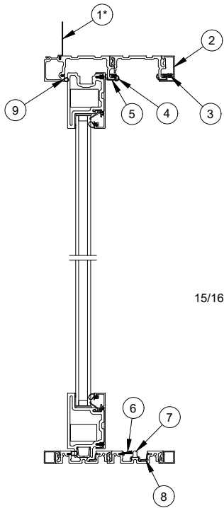
Stationary/Pocket Panel Head Jamb and Sill
