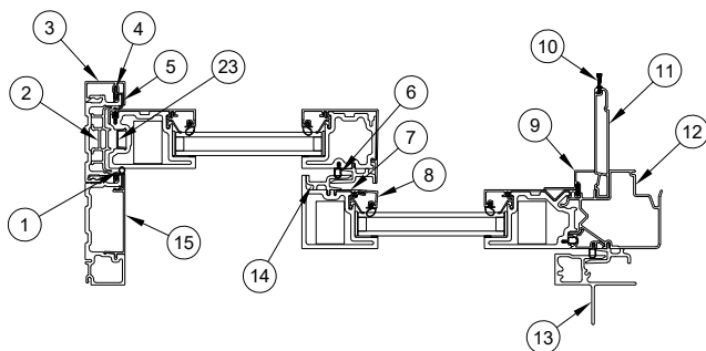
Pocket Uni-directional Jamb Detail
