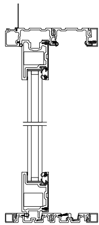
Stationary/Pocket Panel Head Jamb and Sill
