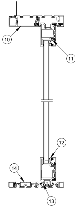
Primary/Inactive Panel Head Jamb and Sill
