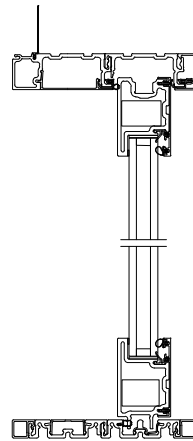
Primary/Inactive Panel Head Jamb and Sill
