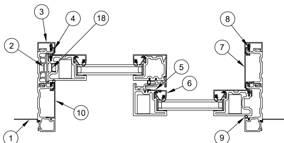
Stacked Uni-directional Jamb Detail
