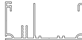
Sill, Frame Sill, Spliced
