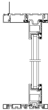
Primary/Inactive Panel Head Jamb and Sill
