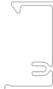
A3248 Frame Liner (Head Jamb and Jamb)
