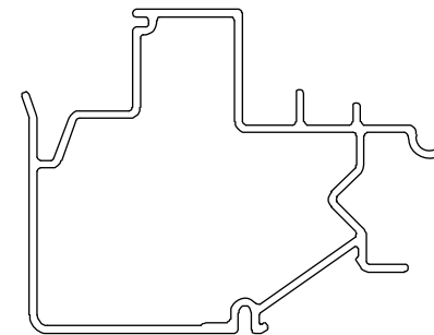
Pocket, Interlock Support Block, A3313
