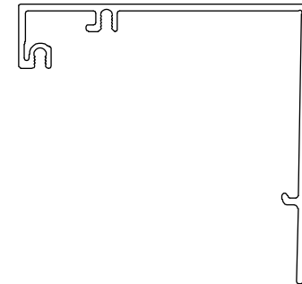
Clad, Interior Interlock Stile, A3363 15/16" Glass
