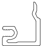
Clad, Exterior Interlock Stile, A3410 15/16" Glass
