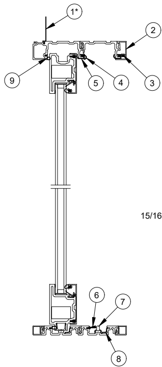
Stationary/Pocket Panel Head Jamb and Sill
