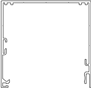
Head Jamb Frame Head Jamb Frame, Spliced
