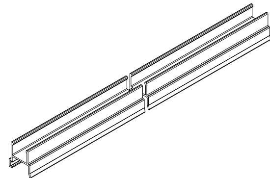
Screen Astragal, A645
