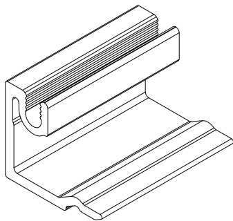
Clad, Exterior Interlock Stile, A3410 15/16" Glass
