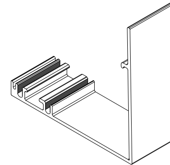
Clad, Interior Interlock Stile, A3350
