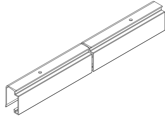
Screen Track Filler, A777 (OX-O, O-XO )
