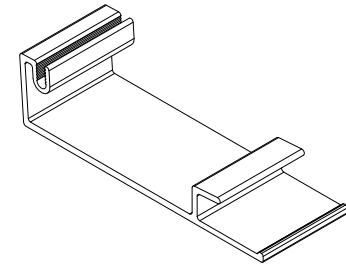
Exterior Sill Cover, A04031
