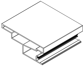
Screen Stop, 6 9/16" ACC, A04145
