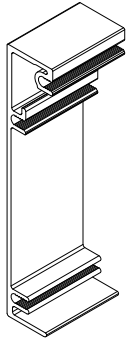
Clad, Locking/Stationary Stile, A3362 15/16" Glass
