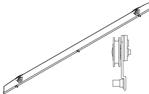
Screen Roller Bar Assembly, A3618
