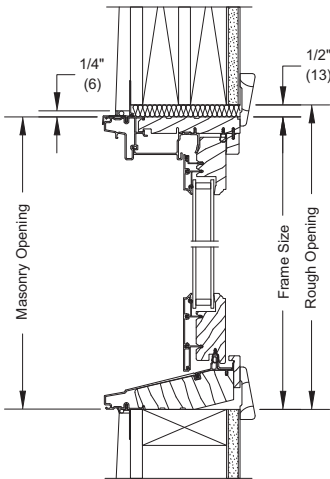
HEAD JAMB AND SILL - PICTURE
