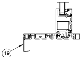
High Performance Sill Option
