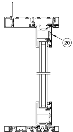
Primary/Inactive Panel Head Jamb and Sill with 1 1/4" Glass
