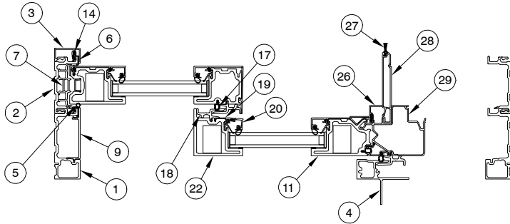
Pocket Uni-Directional Panel 15/16" Glass Jamb
