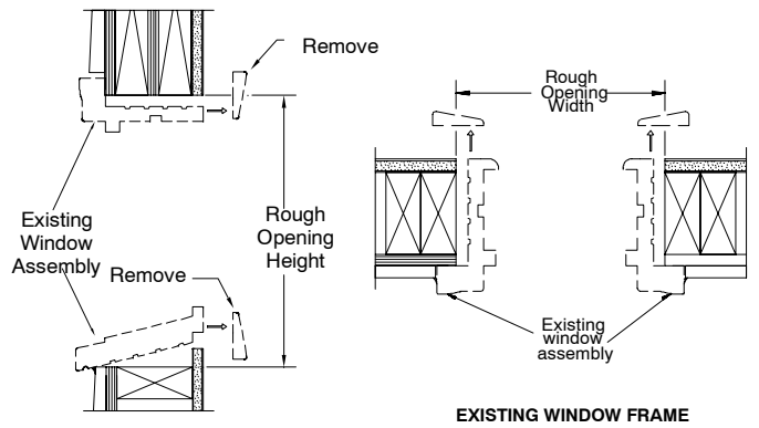
EXISTING WINDOW FRAME
