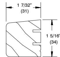
W8653 – Sill Nosing Transom – Pre-June 24, 2013
