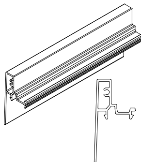
A340 – Mull Cap Hinged Screen
