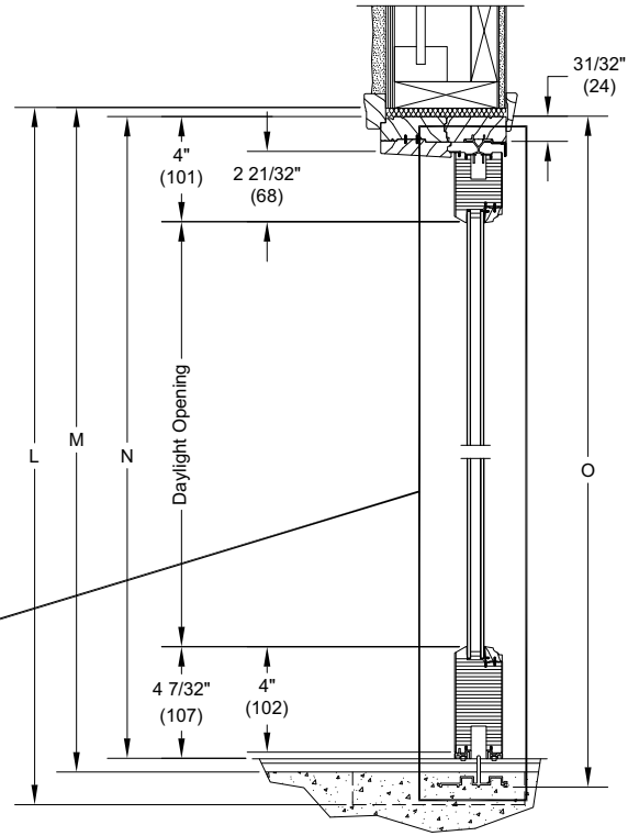
Standard Recessed Sill
