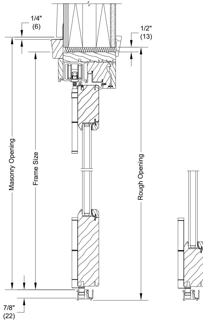
Head Jamb and Floor Channel Sill With Traditional Bottom Rail
