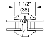
IG ADL For 1 3/4 Doors
