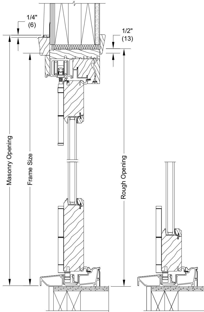
Head Jamb and Standard Sill With Traditional Bottom Rail
