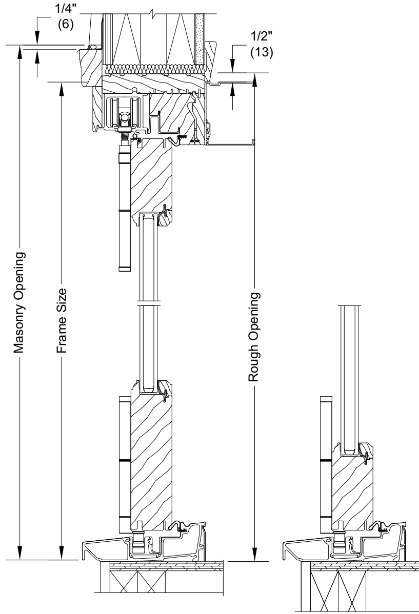
Head Jamb and Standard Sill With Traditional Bottom Rail
