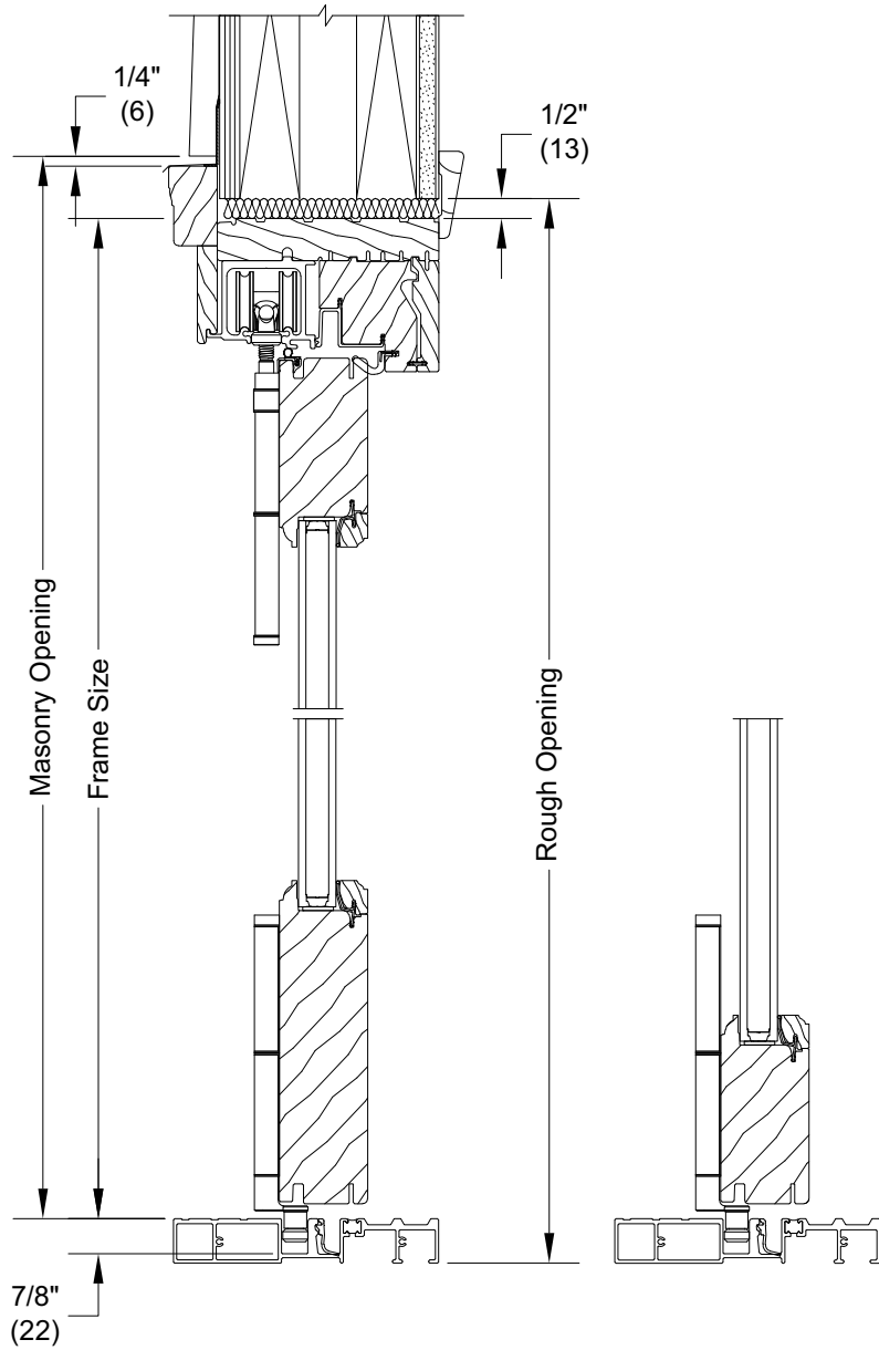
Head Jamb and ADA Sill With Traditional Bottom Rail
