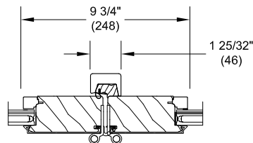
Astragal Detail with Square Sticking
