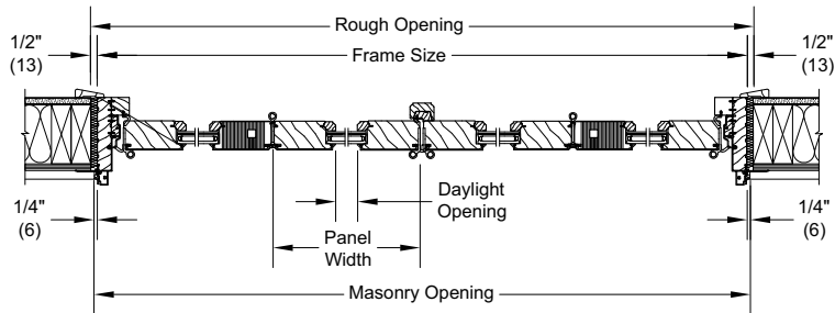
CMOBFD 2L2R
