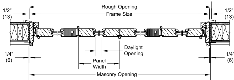
CMOBFD 4L
