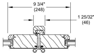
Astragal Detail with Ogee Sticking
