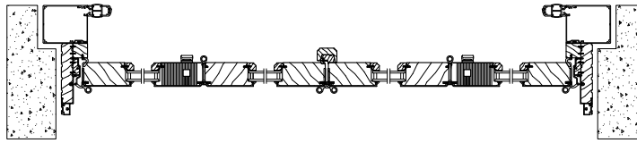
CMOBFD 2L2R
