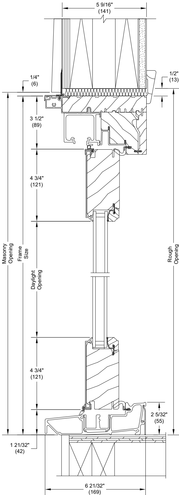
Head Jamb and Sill
