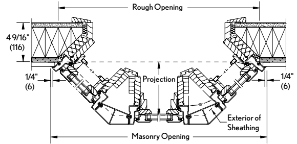
45° Casement Bay with Stationary/Picture Center Unit
