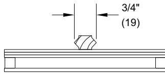
Wood Removable Grille
