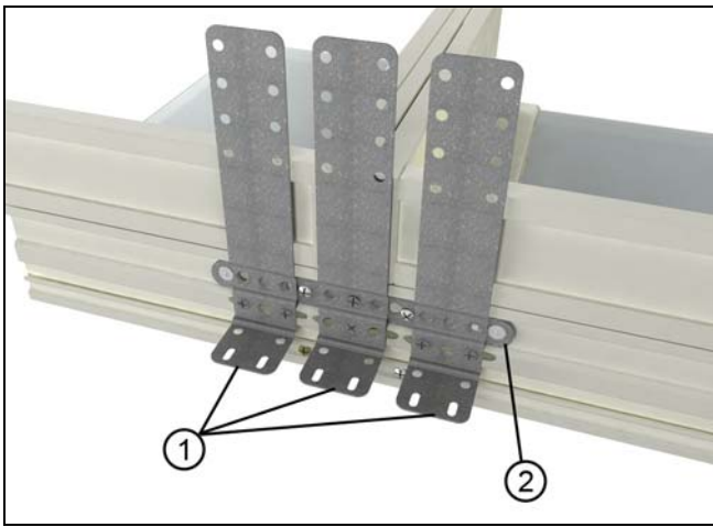
Figure 13 At jamb
