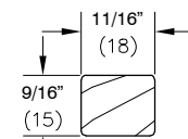
W12495 – Stationary Sweep Filler
