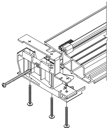
F2050 – 2014 Ultrex Sill, 4 9/16" Jamb's
