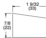
W4098 – Glazing Stop – Front (3/16" Single Glaze)
