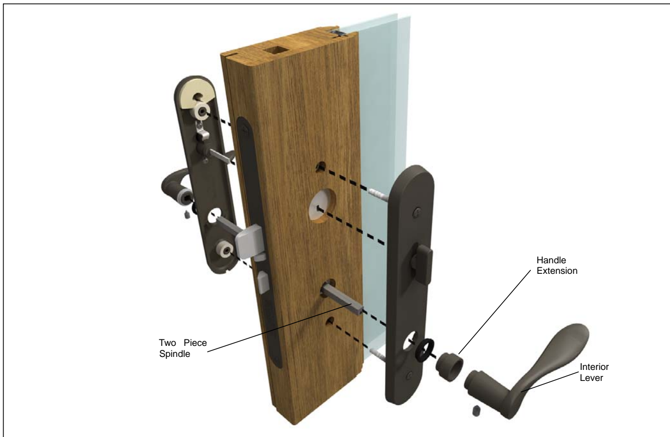
Figure 1 Use the longer two piece spindle and handle extension when installing hardware on doors with interior shades.
